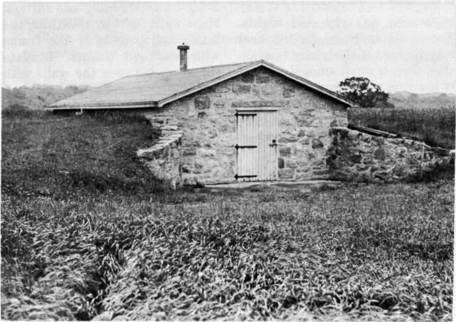
FIGURE 2.—Soil is banked around three walls; the exposed wall has an insulated double door.
