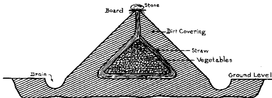
FIGURE 3.—Cone-shaped pit showing details of construction.
