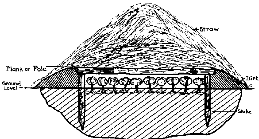
FIGURE 6.—Cabbages are placed upright in a trench that is framed with stakes and covered with straw.
